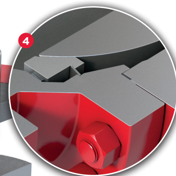
R200 Upstream Seat
