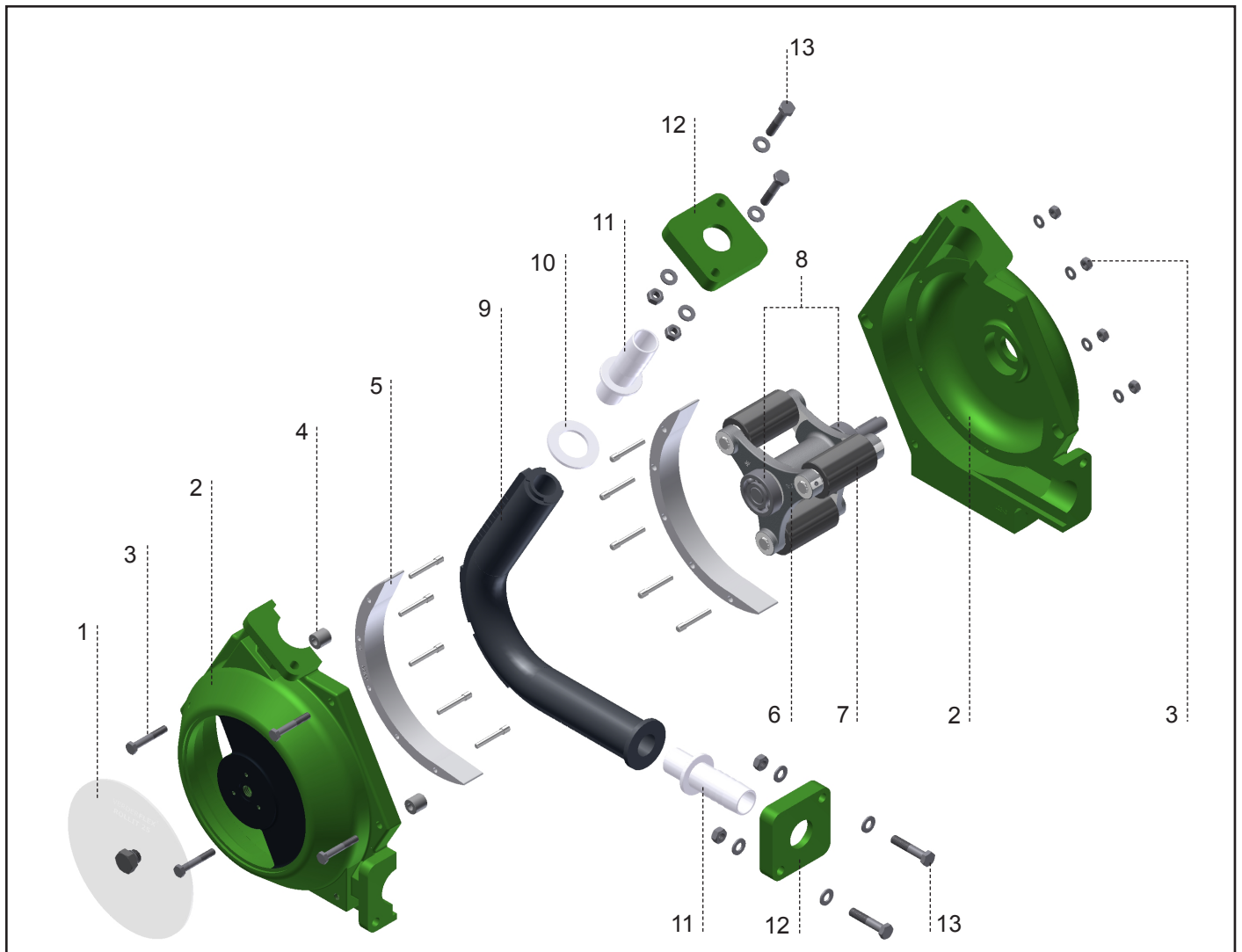
Figure 2 Layout - Rollit 15-50 exploded view
