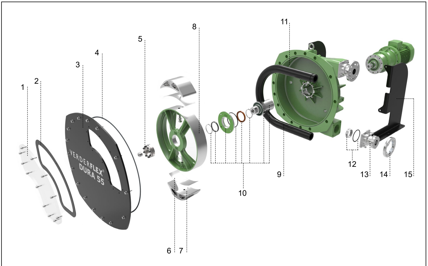
Figure 2 Layout - Dura 55 series - Generic View
