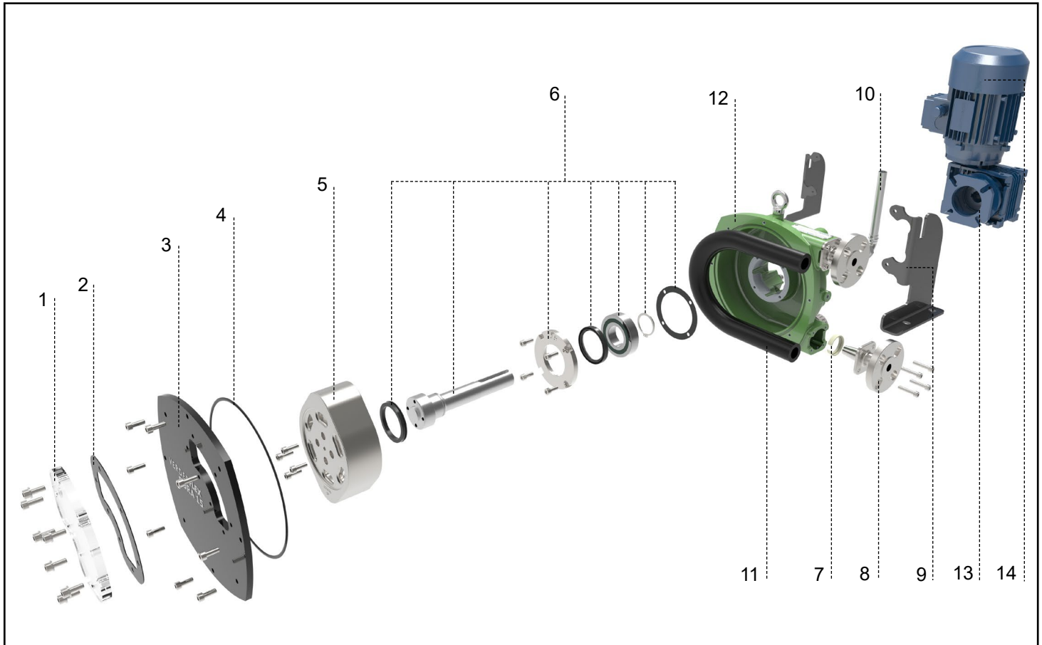
Figure 1 Layout - Dura MK III 10, 15, 25 and 35 Generic View
